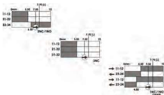
LONG HINGE LEVER WITH RESET
