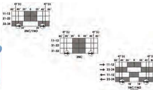
LARGE ROLLER LEVER RESET
