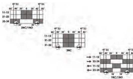
ADJUSTABLE ROLLER LEVER RESET
