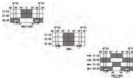
ROLLER LEVER WITH RESET
