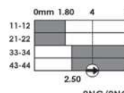
2NC/2NO
