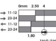
1NC/1NO (SNAP)
