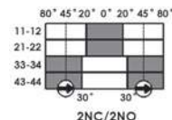
2NC/2NO
