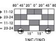
1NC/1NO (SNAP)
