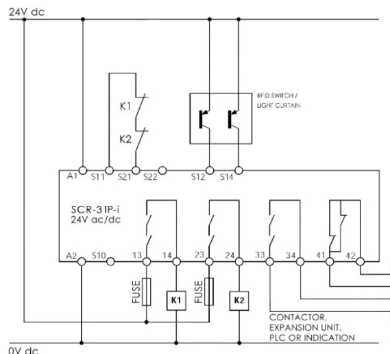
Fig.4 SCR-31P-i, Dual Channel, OSSD Inputs, Auto Reset
